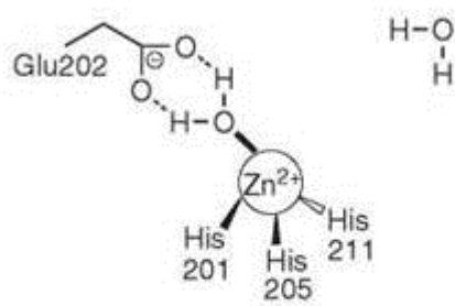
Free enzyme
