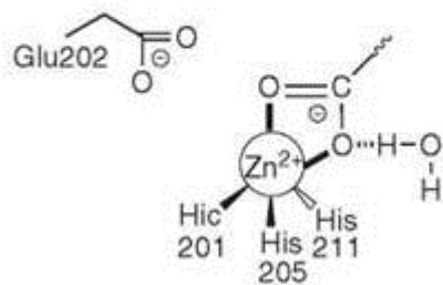
Enzyme-carboxylate complex
