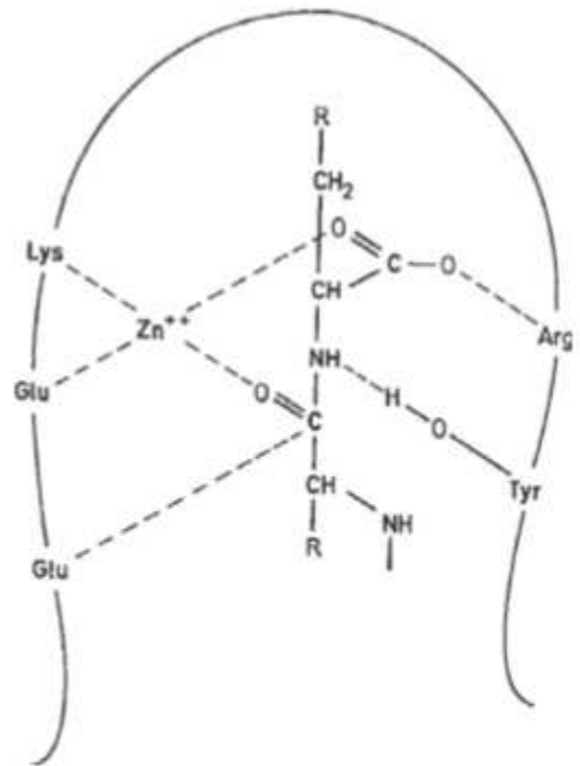
Carboxypeptidase A active site
