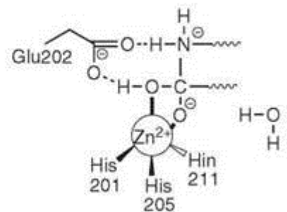
Tetrahedral intermediate
