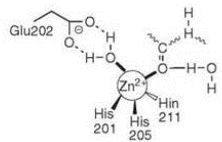
Michaelis complex
